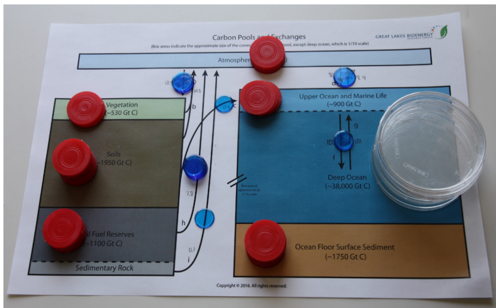
Figure 1: Version 1 models carbon fluxes with poker chips and petri dishes.
